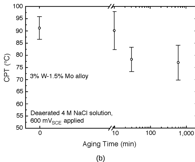
FIGURE 11. Effect of aging at 850^\circ\text{C} on resistance to CPT of: (a) 3% Mo and (b) 3% W-1.5% Mo alloy.
